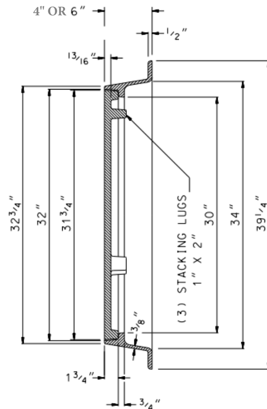
SECTION B-B
