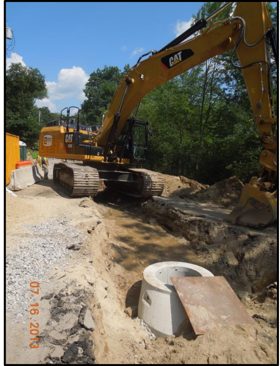
Contractor installing new storm pipe and manhole.
