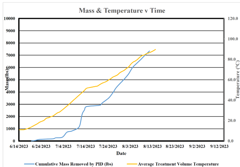
Treatment temperature and contaminant removal over time.
