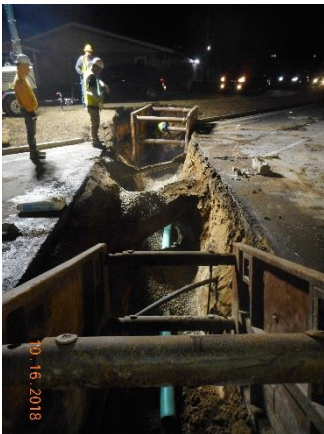
New Sewer Installation
