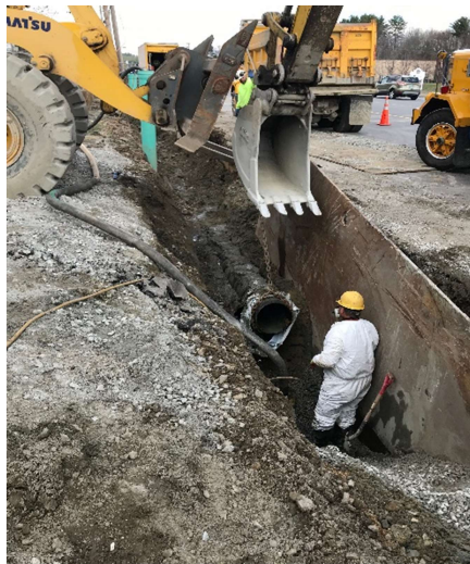
Preparing Water Main Trench
